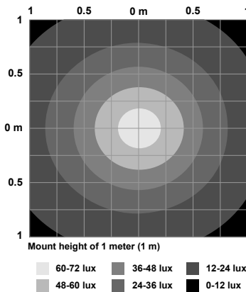
Isolux Pattern
